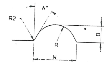
TYPICAL ROUND GROOVES
